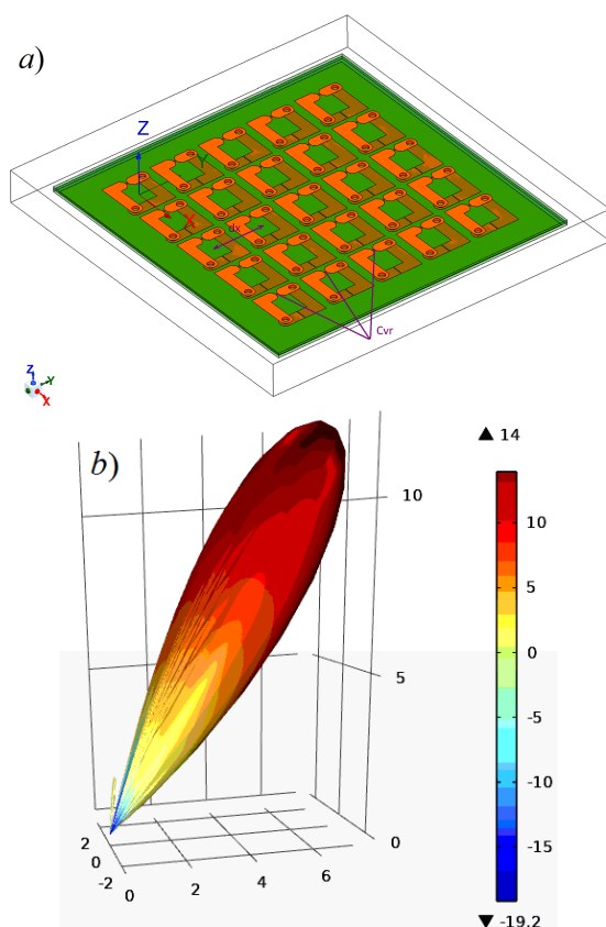
Figure 1.1 – The project of the metamaterial consisting of 25-paired planar spiral resonators located on the dielectric layer ( a ); an example of a radiation pattern diagram formed by the metasurface ( b ).
